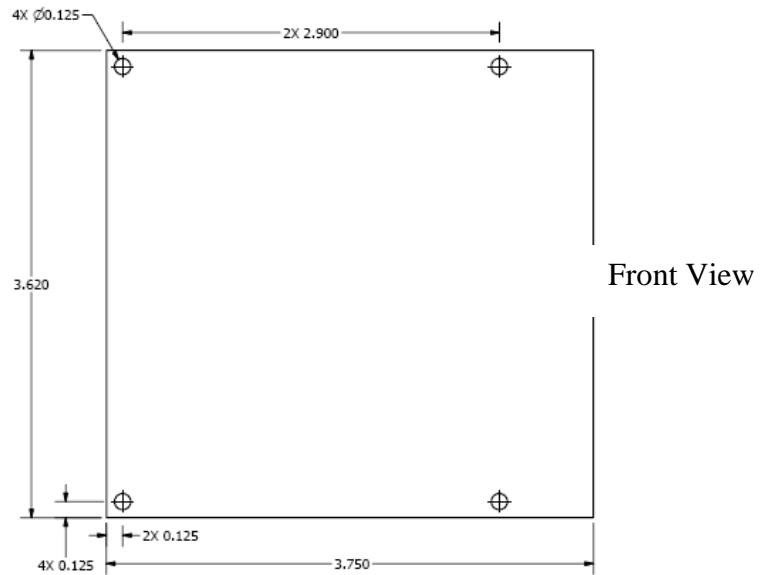
Figure 20 – Board Dimension
